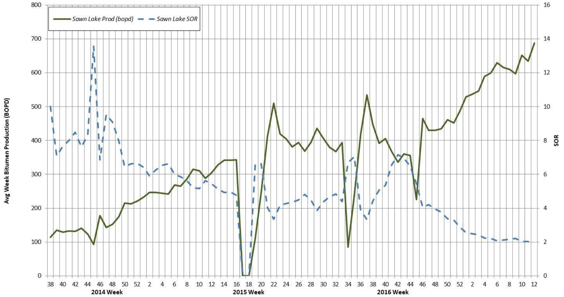
Sawn Lake 1U/1L Production Performance (Weekly Averages)
